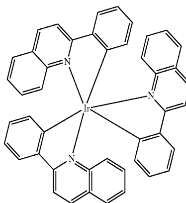
Chemical Formula (5)
