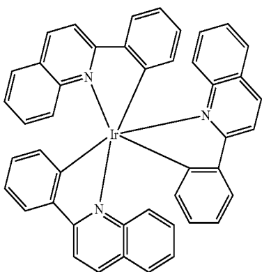
Chemical Formula (5)
