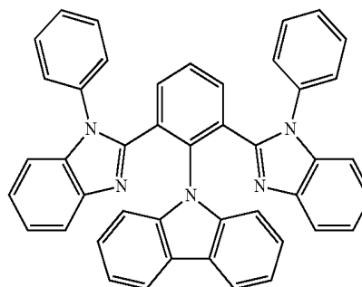
Chemical Formula (2)
